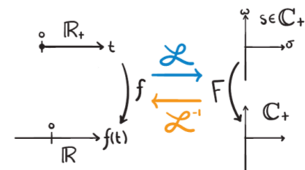
Figure def.2: detail view of Laplace transform maps \mathcal{L} and \mathcal{L}^{-1} along with their image functions f and F .
