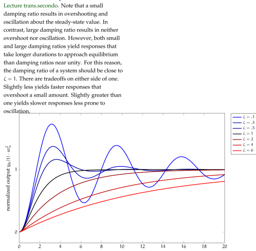
Figure second.2: Forced step response y_o(t) of a second-order system for different values of \zeta . Underdamped, critically damped, and overdamped cases are displayed.
