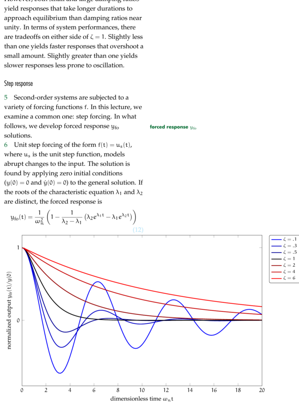
Figure second.1: Free response y_f(t) of a second-order system with initial conditions y(0) and \dot{y}(0) = 0 for different values of \zeta . Underdamped, critically damped, and overdamped cases are displayed.
