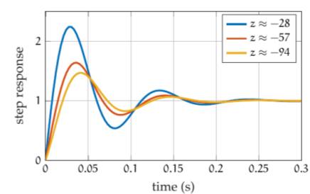
Figure sim.1: step response for different zero locations, from lsim .
